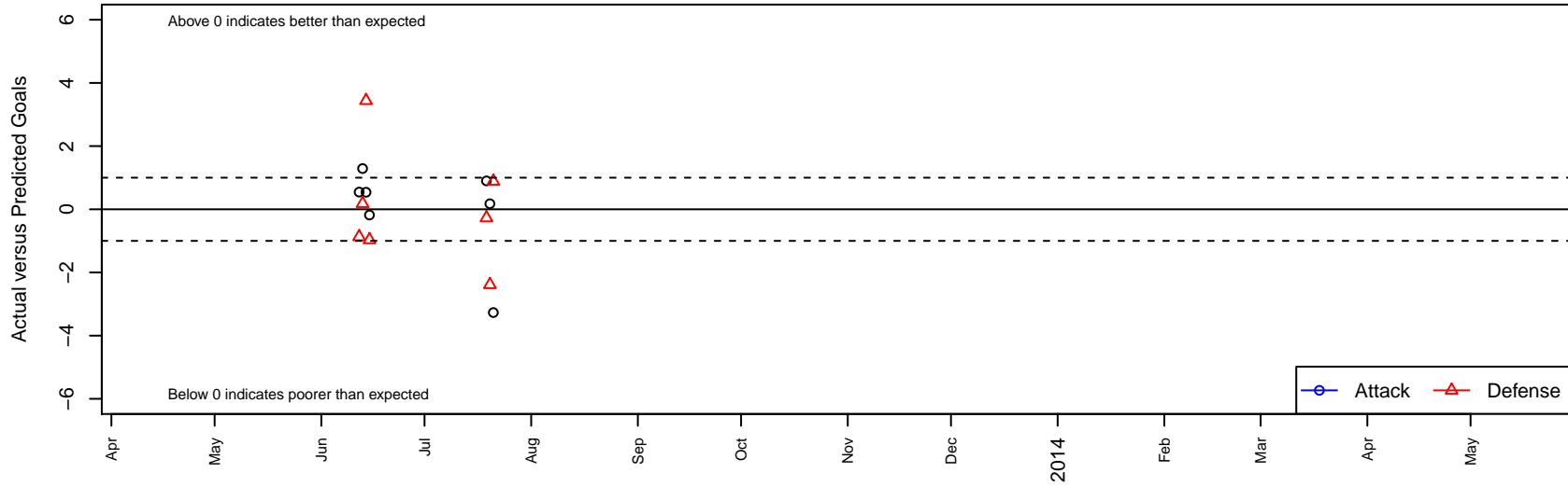
WAFC Pumas B98 Dots are actual minus expected GF (blue circles) and GA (red triangles). Blue line is smoothed change in attack strength. Red is smoothed change in defense strength.
